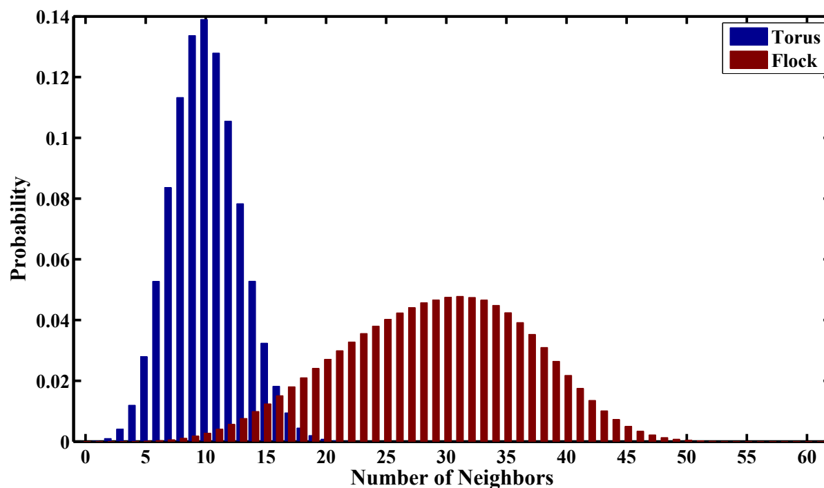
Figure 6.3: Distributions over an agent’s number of neighbors in torus and a flock. N = 100 agents.
